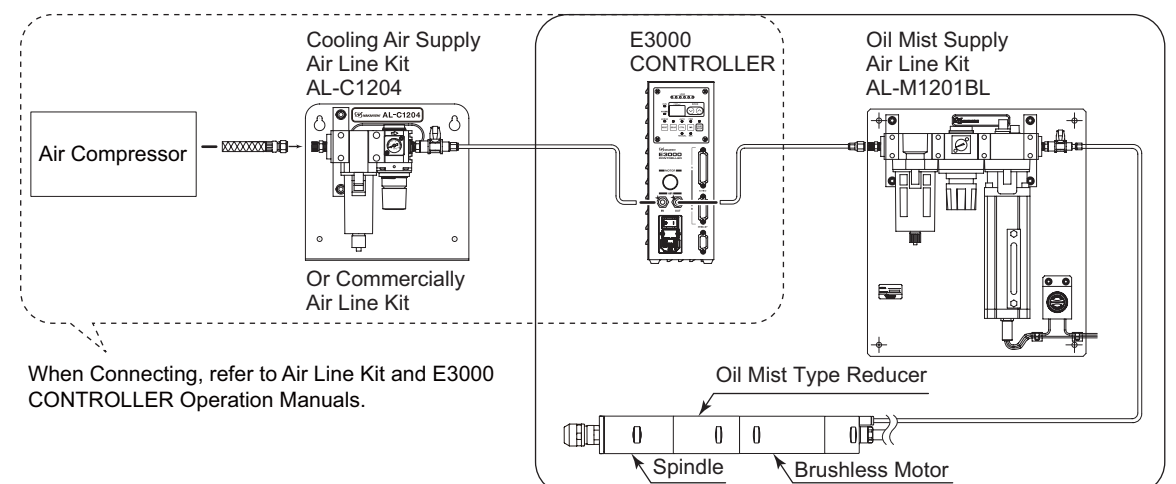
When Connecting, refer to section "6. CONNECTION OF THE MIST AIR LINE KIT (AL - M1201BL) TO THE OIL MIST TYPE REDUCER". Fig. 3
