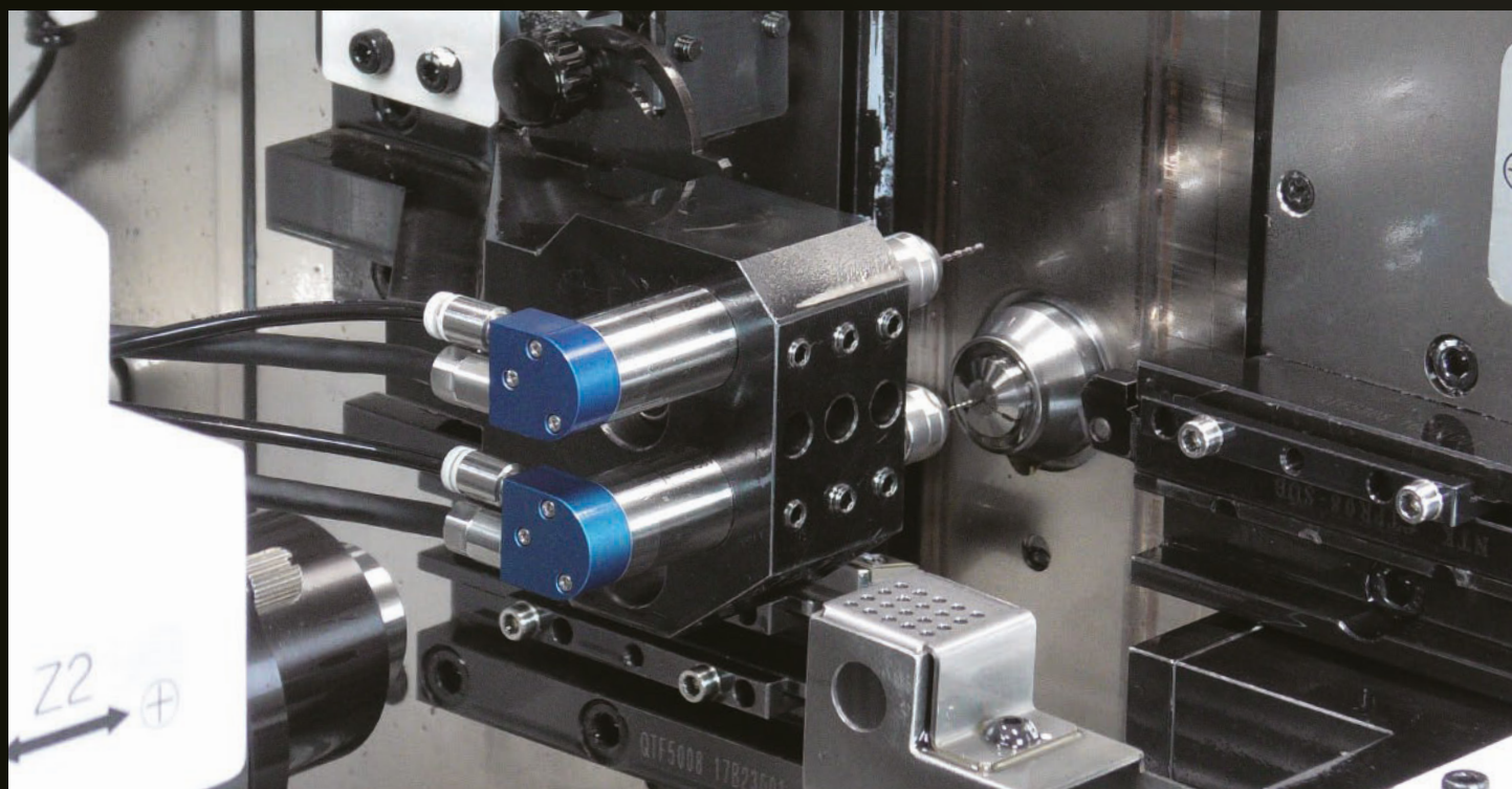
Mounted on Sliding Headstock Type Automatic CNC Lathe: CITIZEN MACHINERY CO., LTD. Cincom R04
